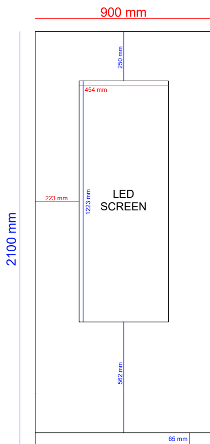
FRONT VIEW
