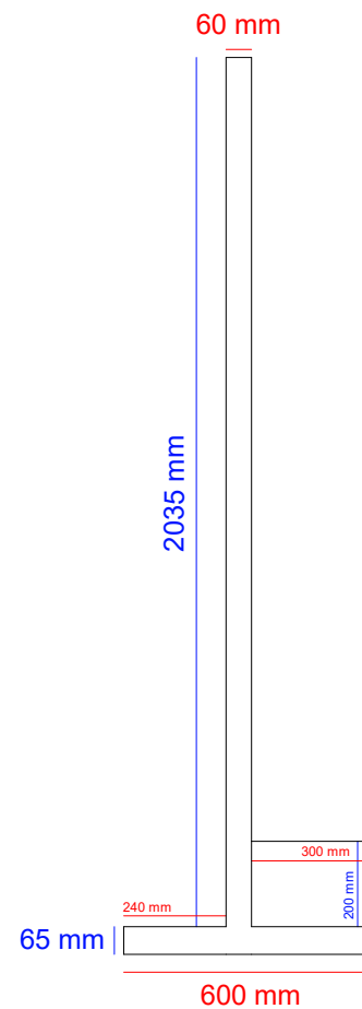
RIGHT
